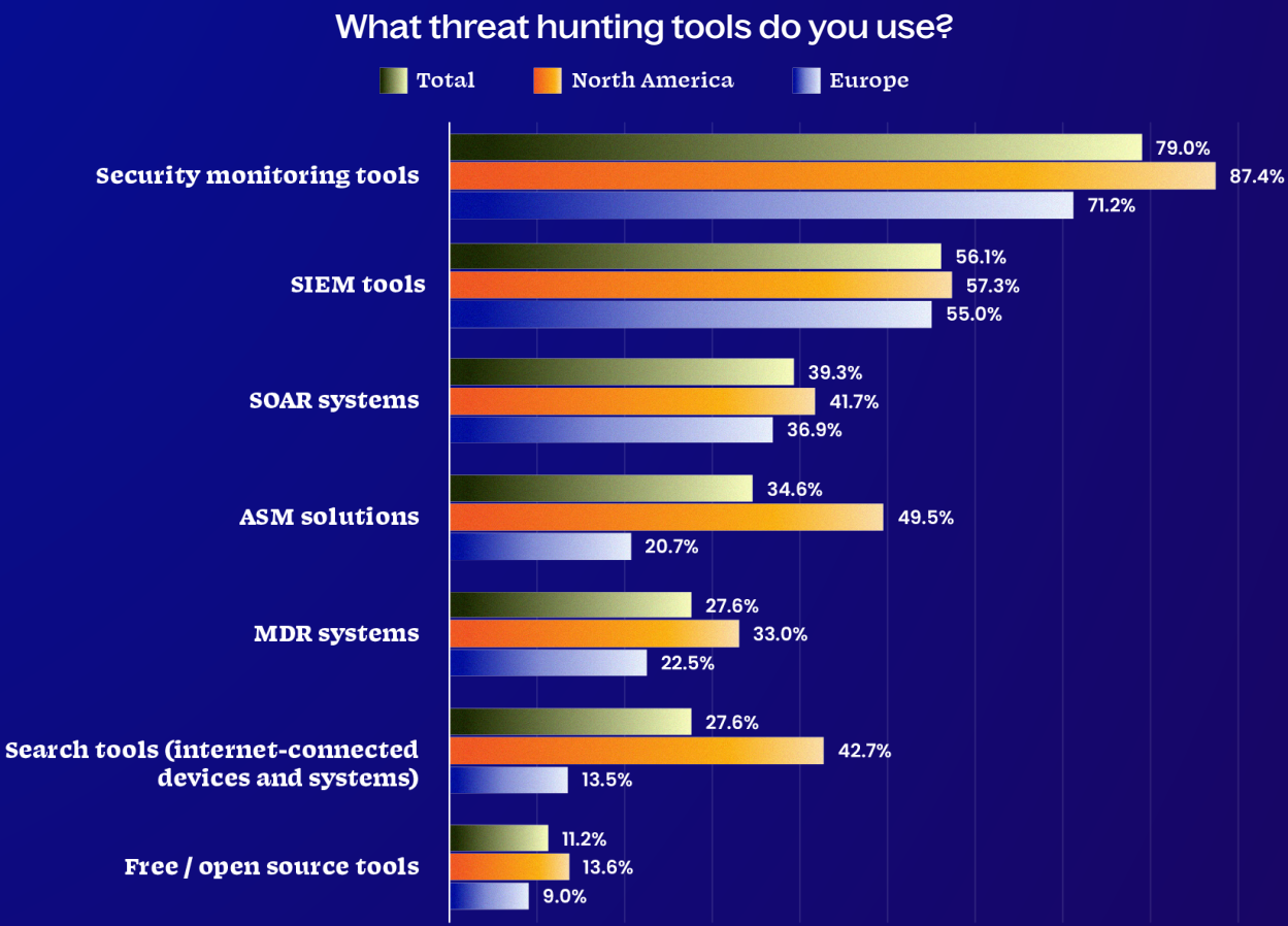
Figure 8: Threat Hunting Tools and Technologies Used
